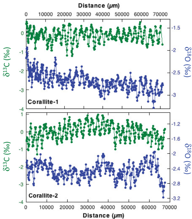
Figure 2. Filtered Goniopora hilli stable isotopic time series. Data suspected of alteration were removed using a standardized filtering method in which the linear approximation for each point was calculated as the linear interpolation of surrounding two points.
