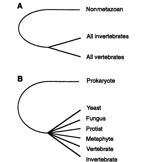
Fig. 3. Relative rate tests. Diagrams illustrate the scheme used to test for homogeneity of sequence divergence rates among metazoan phyla (A) and among eukaryotic kingdoms (B). The test results (Tables 3 and 4) indicate similar branch lengths and therefore similar rates of sequence divergence in both cases.
